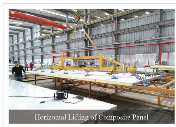
AC-Vacuum Lifter (14 Suckers) FS-WBSJ1500-14S (1500KG)
