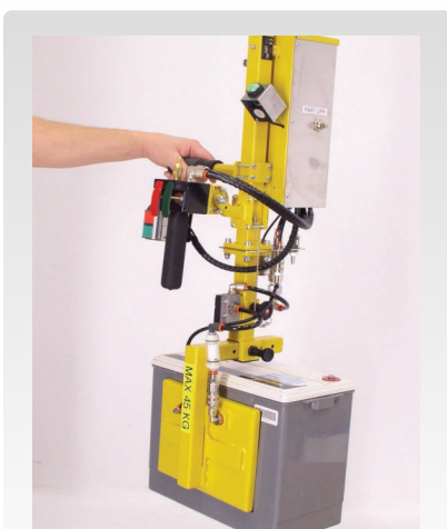
TOOL NÂNG ẮC QUY, PIN A combi-gripper for batteries
