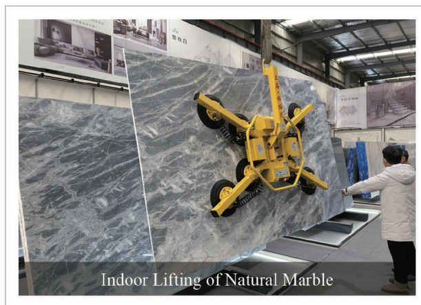
DC-Vacuum Lifter (8 Suckers) FS-MSFX800-8S (800KG)
