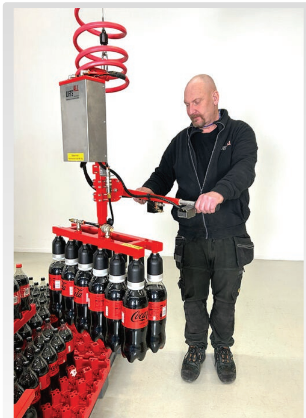
TOOL NÂNG NƯỚC ĐÓNG CHAI Lifting tool for Plastic Bottles
