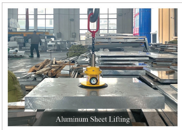
Mechanical Vacuum Lifter (Single Sucker) FS-WDL80-IS (80KG)
