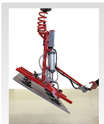
TOOL NÂNG TẤM Tool for picking up barrle
